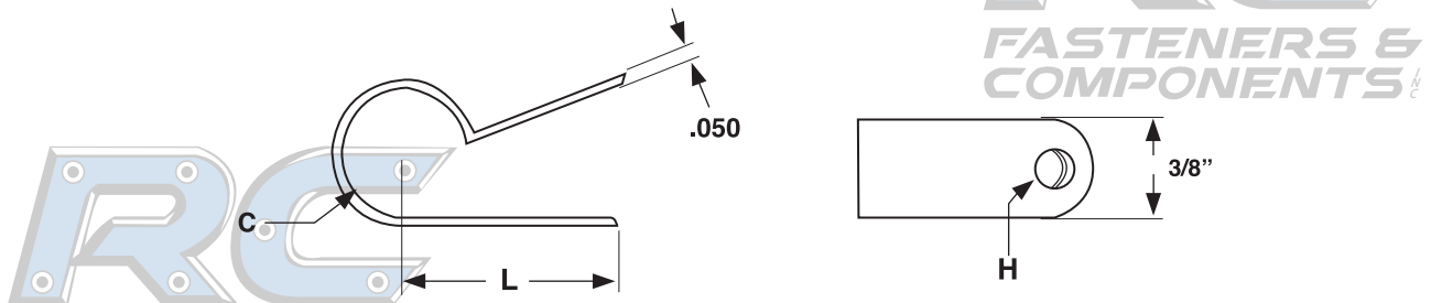
NYLON STANDARD CABLE CLAMPS — 3/8" WIDE CONTACT AREA
